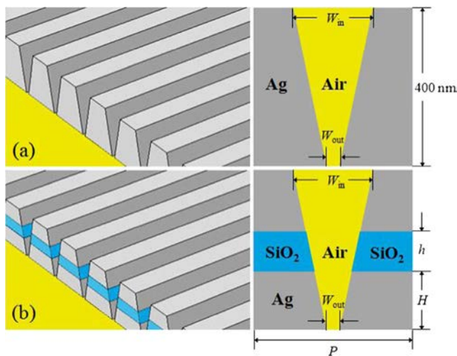
Fig. 1 Schematics of the tapered monolayer slits (a) and the tapered multilayer slits (b)
