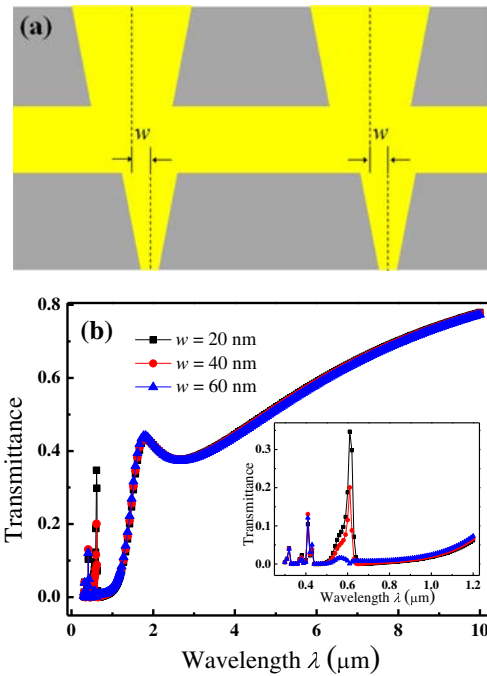
Fig. 8 (a) Schematic of the tapered multilayer slits in which the centers of two separated monolayer slits deviate; (b) Simulated transmission spectra of the tapered multilayer slits with different w values
