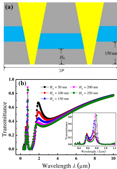
Fig. 7 (a) Schematic of the tapered multilayer slits with asymmetric layer heights; (b) Simulated transmission spectra of the tapered multilayer slits with different H_V values
