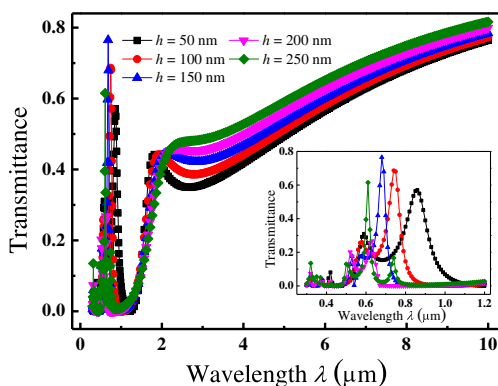
Fig. 4 Simulated transmission spectra of the tapered multilayer slits with different h values
