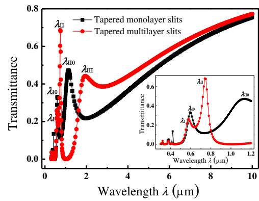
Fig. 2 Simulated transmission spectra of the tapered monolayer slits and the tapered multilayer slits
