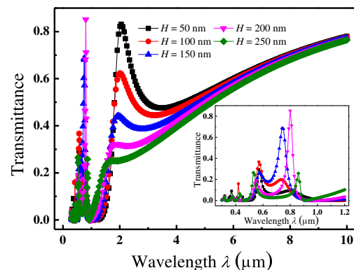
Fig. 5 Simulated transmission spectra of the tapered multilayer slits with different H values
