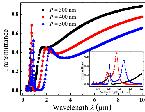
Fig. 6 Simulated transmission spectra of the tapered multilayer slits with different P values
